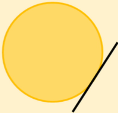
Tangent
