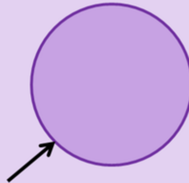
Circumference
