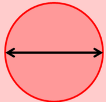
Diameter
