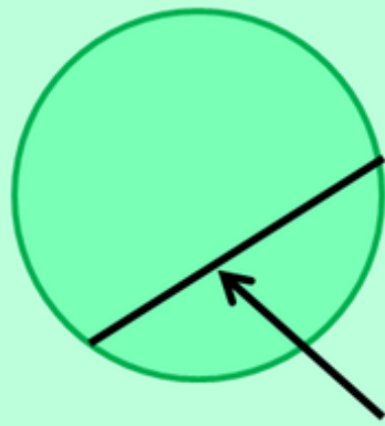
Chord
